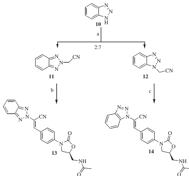
Scheme 3. Reagents and conditions: (a) ClCH 2 CN, TEA, DMF, 110°C, 50%; (b) ald. 1 , benzoic acid, piperidine, toluene, reflux, 40%; (c) same as (b), 50%.
