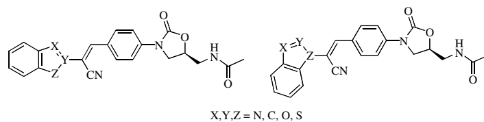
Scheme 3. Reagents and conditions: (a) ClCH 2 CN, TEA, DMF, 110°C, 50%; (b) ald. 1 , benzoic acid, piperidine, toluene, reflux, 40%; (c) same as (b), 50%.
